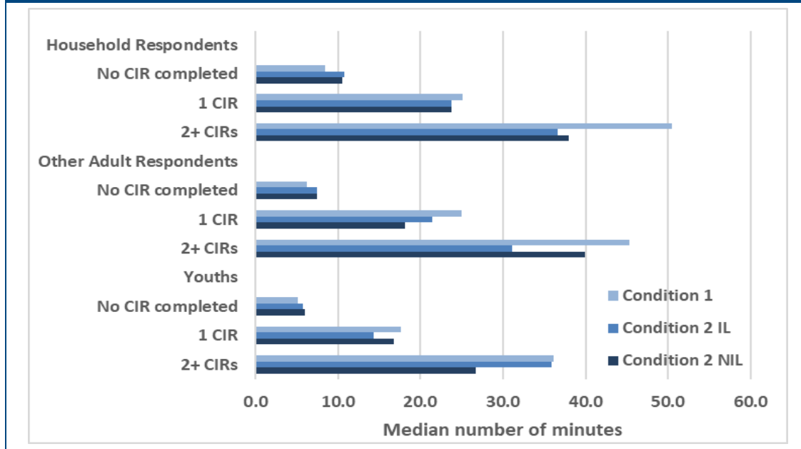
Figure 6-3. Median time to complete the Person Interview by number of CIRs, Condition 1, Condition 2 IL and NIL
