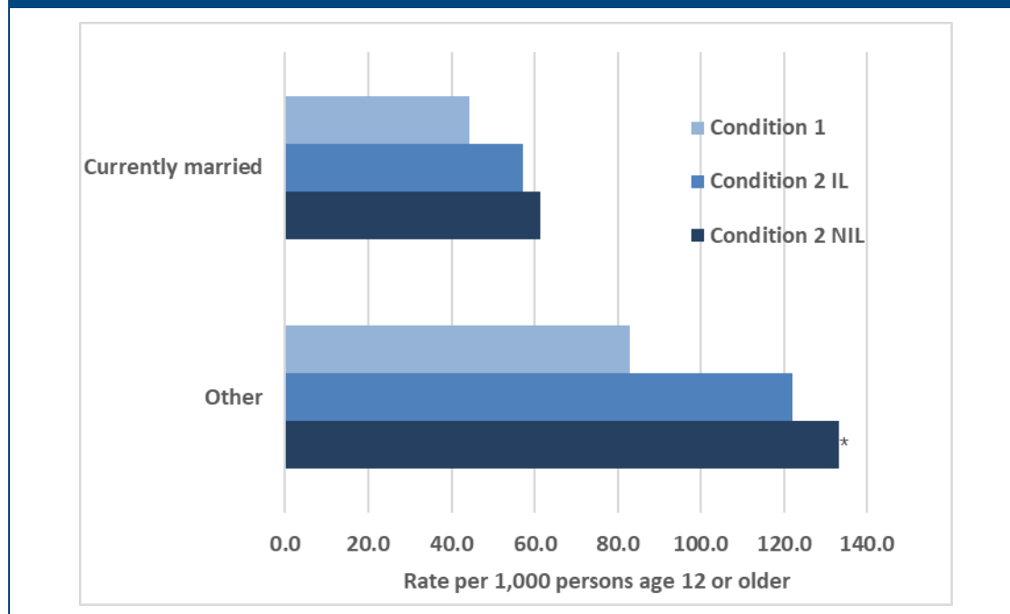
Figure 3-6. Violent victimization rate by marital status, Condition 1 and Condition 2 IL and NIL
