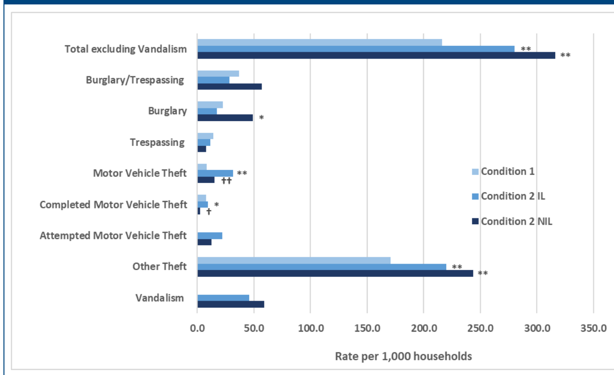
Figure 4-3. Victimization rates by type of property crime, Condition 1 and Condition 2 IL and NIL
