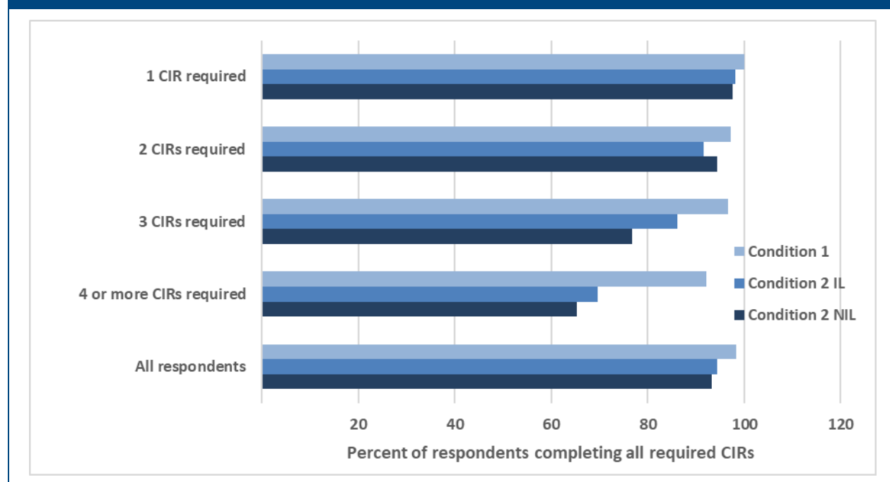
Figure 5-3. Percentage of respondents with all requested CIRs considered complete by number requested, Condition 1 and Condition 2 IL and NIL
