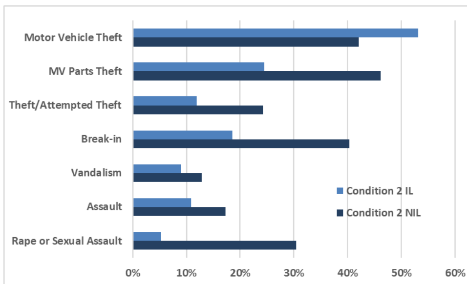
Figure 7-1. Percentage (unweighted) of reported victimizations with two or more screener TOC flags, by screener series where victimization was initially reported, Condition 2 IL and NIL
