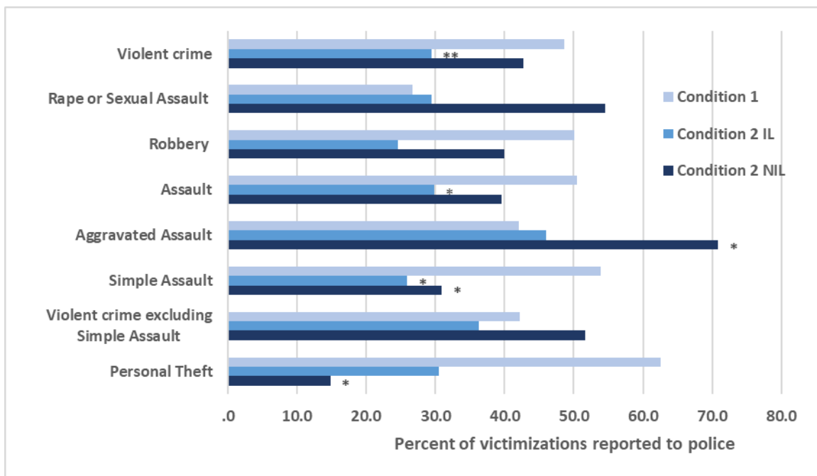
Figure 4-8. Percentage of violent crimes reported to the police, Condition 1 and Condition 2 IL
