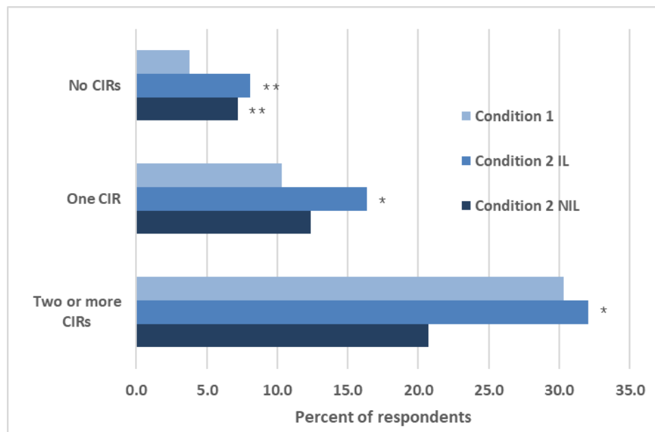
Figure 6-8. Percent of respondents reporting the survey was too long by number of CIRs completed, Condition 1 and Condition 2 IL and NIL
